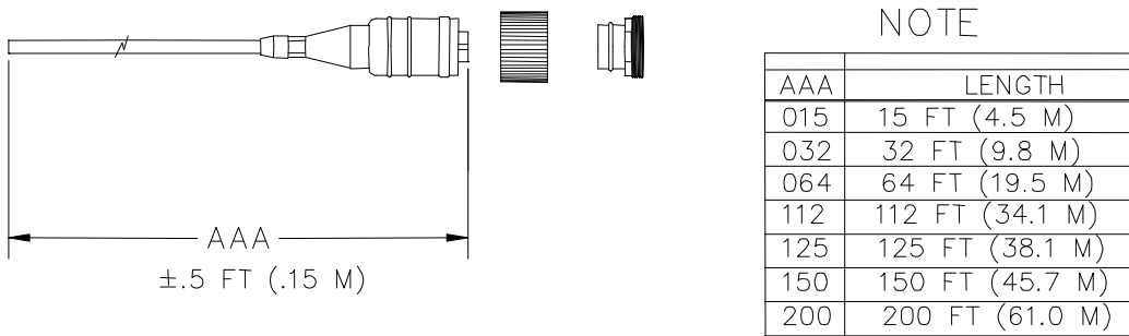
Figure 6: Splash Proof Interconnect Cable
